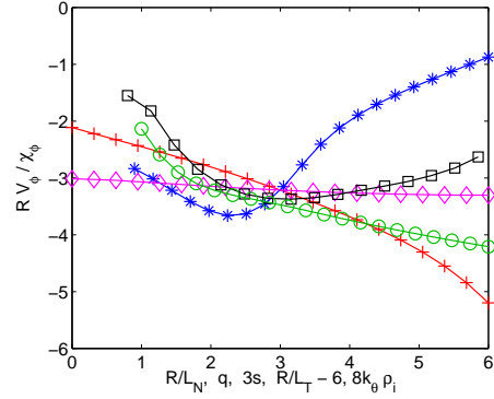
FIG. 2: RV_\phi/\chi_\phi as a function of R/L_N (+), 3\hat{s} (*), q (o), and R/L_T - 6 (diamonds), and 8k_\theta\rho_i (squares)
