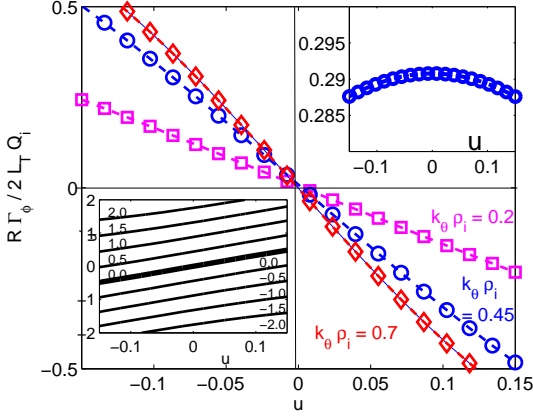
FIG. 1: (R/2L_T)\Gamma_\phi/Q_i as a function of u for three values of k_\theta\rho_i : 0.45 (o), 0.2 (squares), and 0.7 (diamonds). The top right graph shows the growth rate as a function of u and the down left graph the contour lines of (R/2L_T)\Gamma_\phi/Q_i as a function of u and u' , for k_\theta\rho_i = 0.2 and 0.5 respectively.
