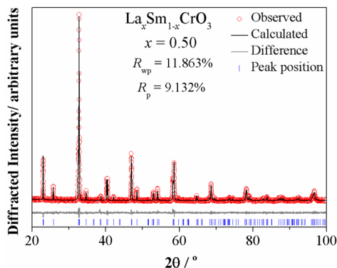
Figure 3. Rietveld refinement against high-resolution PXRD patterns of the hydrothermally synthesized mixed rare-earth orthochromite \text{La}_x\text{Sm}_{1-x}\text{CrO}_3 solid solution x = 0.5 . Observed (red circles), calculated (black line), difference (gray line), and peak position (blue tick marks) data calculated from the refinement are shown.
