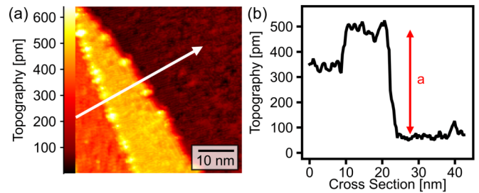
FIG. 11. (a) CCT image taken at 0.8 V/0.1 nA of two steps, one of about 1.3 Å height and one of a bulk lattice constant height, as shown in the height profile in (b).
