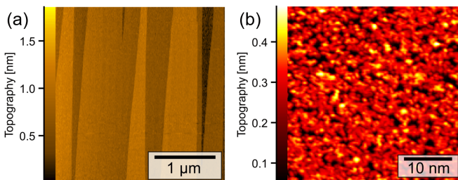
FIG. 10. (a) (001) surface of cleaved LaB 6 as observed with AFM under ambient conditions. (b) CCT of a disordered surface area taken at 1 V/0.1 nA.
