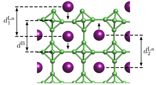
FIG. 15. Structure relaxation at the slab surface. d^{\text{La}} are distances between La atoms of the topmost layers as indicated. d^{\text{B}} is the distance between the centers of mass of the two octahedra. The small black arrows indicate the direction of the relaxation movement compared to the bulk structure.
