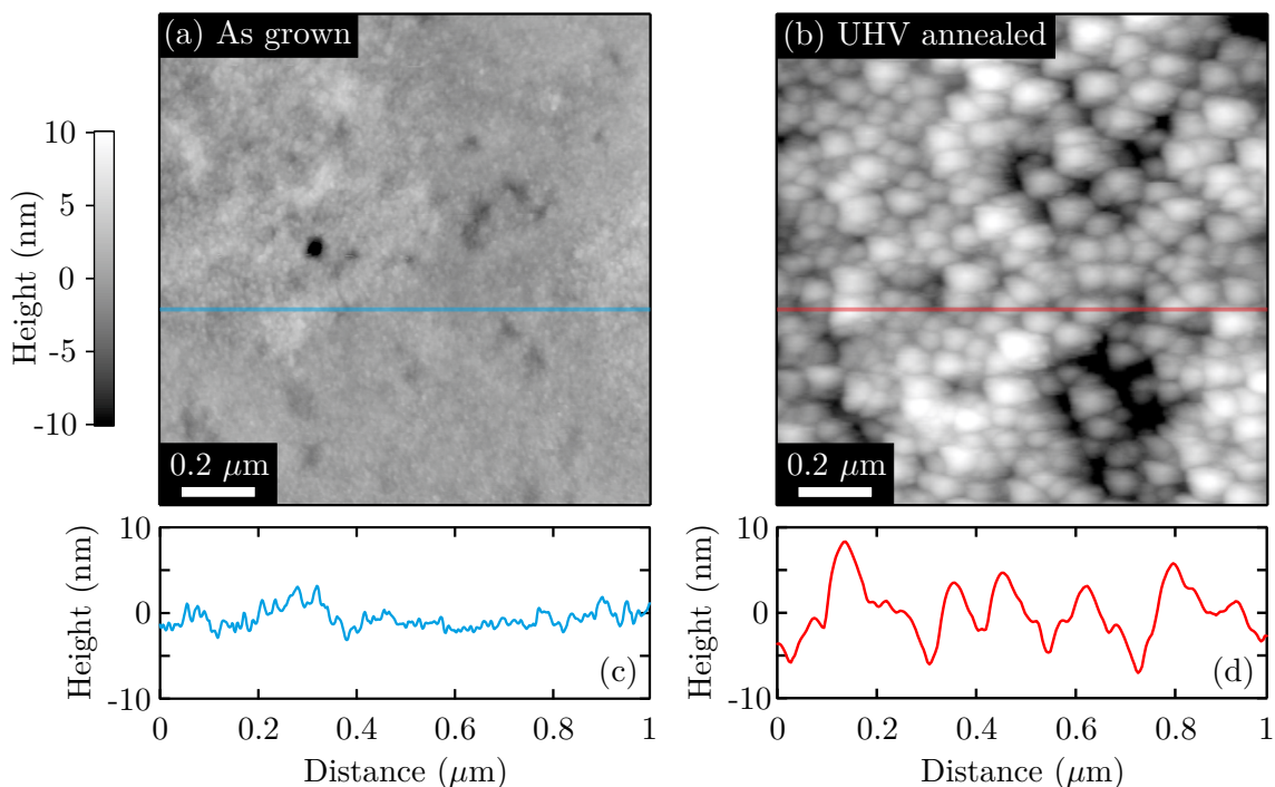
Figure 2.17. AFM data illustrating the effect of UHV annealing on the CdO(100) surface. (a) and (b) show 1 \mu\text{m} \times 1 \mu\text{m} AFM height images of an as-grown and UHV annealed CdO(100) sample, showing the surface roughening and recrystallisation following UHV annealing. Both images are shown with the same indicated colour scale to allow the difference to be observed. (c) and (d) show line profiles taken from the positions indicated across images (a) and (b) to allow the surface roughness to be observed.
