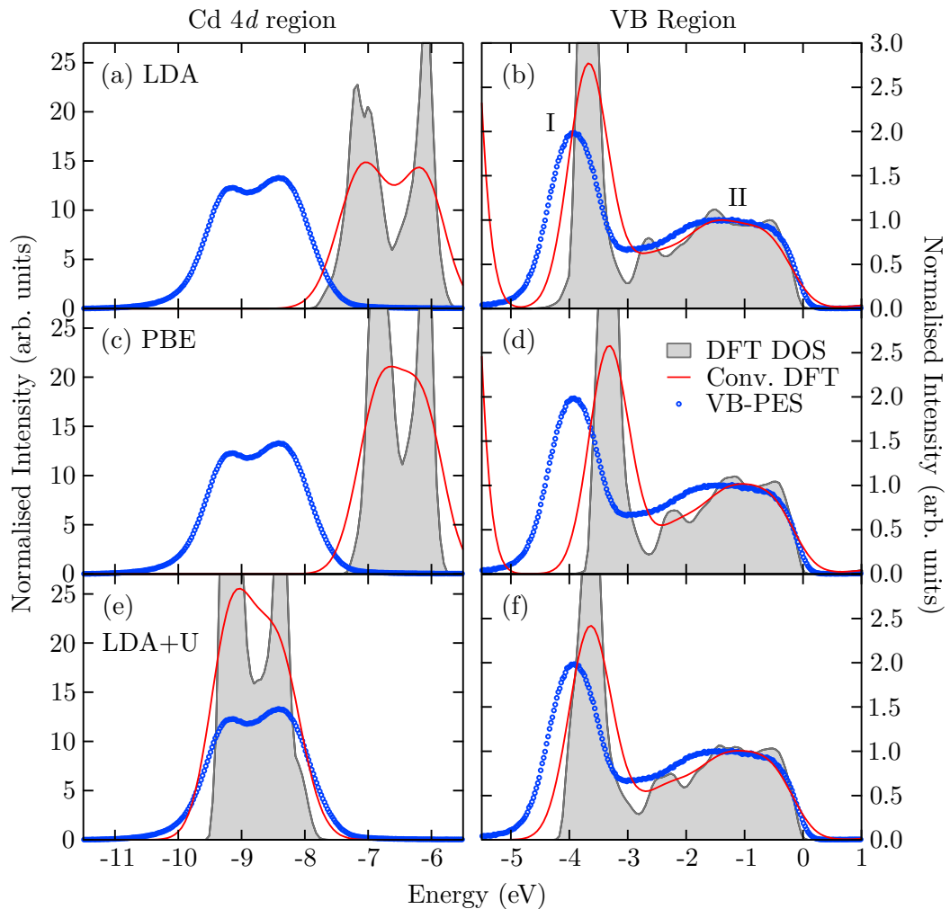
Figure 5.5. VB and Cd 4 d PES spectra compared to DFT, (a) and (b) LDA, (c) and (d) PBE, (e) and (f) LDA+ U . The DFT PDOS are weighted by the photoionisation cross-sections and summed, shown by the gray shaded areas. The weighted PDOS after convolution with a 0.7 eV FWHM Gaussian are shown by the red line. The experimental data (blue circles) shown is taken with h\nu = 6054 eV, and a Shirley background has been subtracted. I and II are peak labels. All energy scales are referenced to the VBM. The experimental spectra and convolved DFT are normalised to the maximum of VB peak II, and the same normalisation has been applied to both the VB and Cd 4 d regions. Note the different intensity scales.
