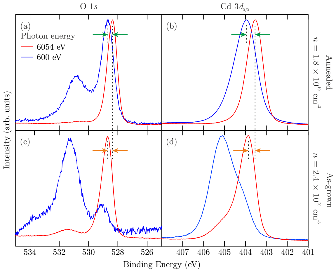
Figure 4.4. Comparison of HAXPES (red) and SXPES (blue) spectra taken with h\nu = 6054 eV and h\nu = 600 eV respectively. (a) O 1s , (b) Cd 3d_{5/2} for the annealed sample ( n = 1.8 \times 10^{19} \text{ cm}^{-3} ). (c) O 1s , (d) Cd 3d_{5/2} for the as-grown sample ( n = 2.4 \times 10^{20} \text{ cm}^{-3} ). The peak shifts indicated by the green arrows are assigned to surface band bending effects, and the orange arrows to CB filling as discussed in the main text.
