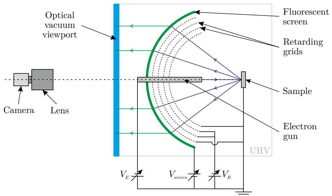
Figure 2.15. Schematic of a reverse-view LEED optics, with the key components labeled. The electron gun provides an incident beam of electrons at an energy set by ( V_E ). These electrons travel through the field free region, established by grounding both the sample and inner most grid, and diffract from the sample surface. To filter out the inelastically scattered electrons, a retarding voltage ( V_R ) is applied just below the beam energy. The elastically diffracted electrons are then accelerated into the fluorescent screen, from where they can be imaged using a camera. The optics need to be operated in UHV conditions.
