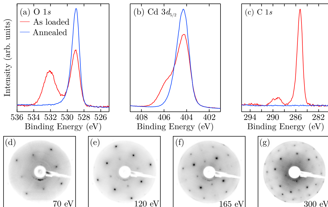
Figure 2.16. (a-c) A comparison of XPS spectra for as-loaded and UHV annealed CdO(100) samples, taken with h\nu = 1486.6 eV. The spectra have been normalised to the Cd 3d_{5/2} area, and the annealed spectra shifted by -1.08 eV to align the peaks, allowing the cleaning effect to be clearly observed. (d-g) show typical LEED images taken from an UHV annealed CdO(100) sample, with the sharp (1 \times 1) pattern indicating a well ordered surface. The images have been inverted to improve contrast.
