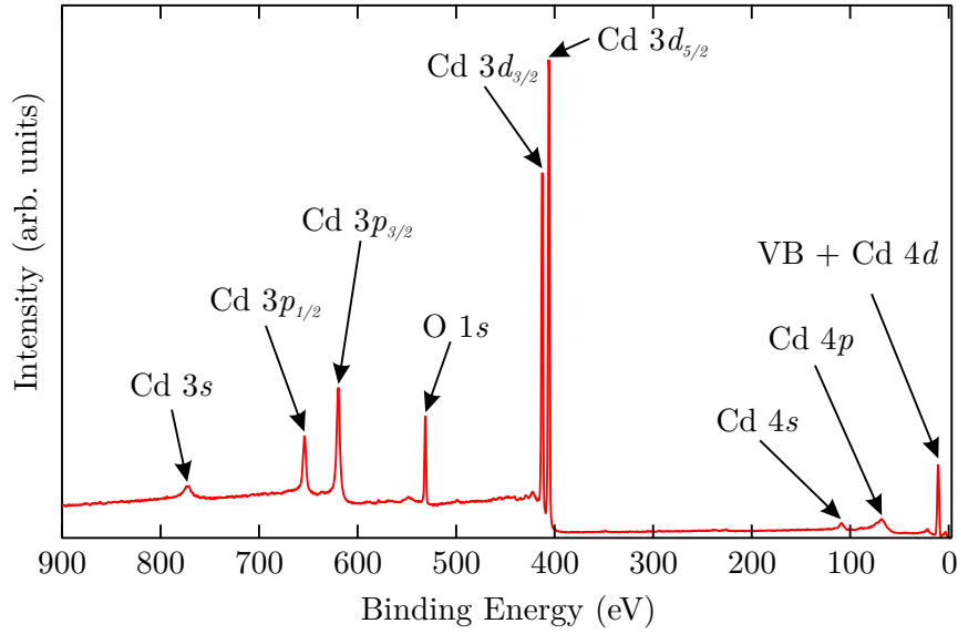
Figure 2.3. An example XPS survey spectra of a clean CdO surface, obtained at the Warwick XPS facility. The sample was illuminated by monochromated Al K_{\alpha} ( h\nu = 1486.6 eV) radiation. An analyser angular acceptance of \pm 7^{\circ} and a pass energy of 50 eV were employed.
