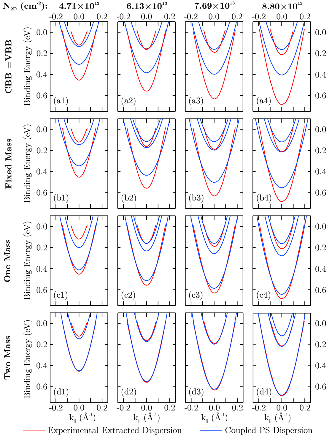
Figure 6.8. Results of fitting the coupled Poisson-Schrödinger model to the extracted subband dispersions. The experimentally extracted dispersions are shown in red for each of the 2D electron densities, and the simulated subband dispersions are shown in blue. Four approaches to the fitting are shown as described in the text, with the numerical results given in table 6.3. Rows: (a) CBB=VBB, (b) m^* = 0.24m_e , (c) m^* is a fitting parameter, (d) the subband effective mass is allowed to vary, while the bulk mass is set at m^* = 0.24m_e . Columns: (1) N_{2D} = 4.71 \times 10^{13} cm -2 , (2) N_{2D} = 6.13 \times 10^{13} cm -2 , (3) N_{2D} = 7.69 \times 10^{13} cm -2 , (4) N_{2D} = 8.80 \times 10^{13} cm -2 .
