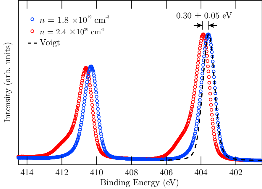
Figure 4.6. HAXPES Cd 3d spectra for both as-grown ( n = 2.4 \times 10^{20} \text{ cm}^{-3} ) and annealed ( n = 1.8 \times 10^{19} \text{ cm}^{-3} ) CdO samples. A symmetrical Voigt peak fitted to the low BE side of the Cd 3d_{5/2} is also shown to allow the asymmetry to be observed.
