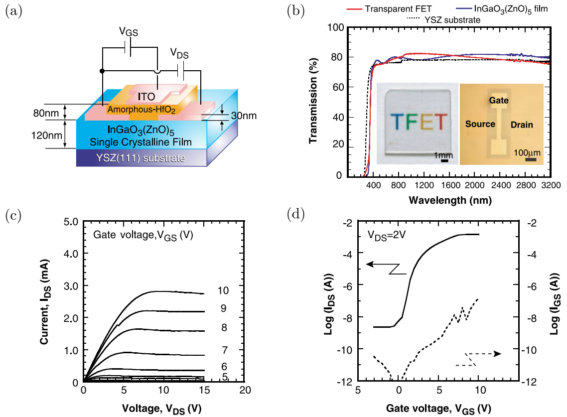
Figure 1.1. A transparent field effect transistor (TFET). (a) Schematic of the TFET device structure (b) Optical transmission spectra of the TFET, the YSZ substrate and \text{InGaO}_3(\text{ZnO})_5 layer for comparison. (c) and (d) Output characteristics of the TFET indicating an on-off current ratio of \sim 10^6 . Figure adapted from [13].
