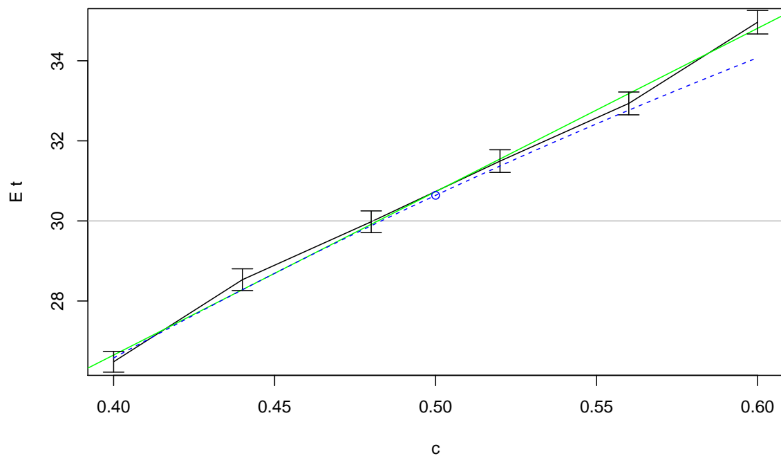
Figure 2: Fitting the Strauss model (1). The top figure shows the average of 100 simulations at five values of c . The lower figure shows the means and 95% confidence intervals based on 1000 simulations at six values of c , plus (green) the fitted regression line and (blue, dashed) values estimated by polysampling from 1000 simulations at c = 0.5 . The grey line is the observed value.
