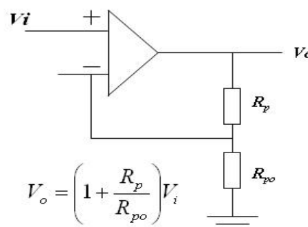
Figure 1. Non-inverting amplifier circuit.
