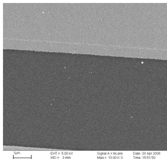
Figure 3. Micrograph of self-assembled AuNT film showing good homogeneity including coverage of the gold electrodes (brighter areas).
