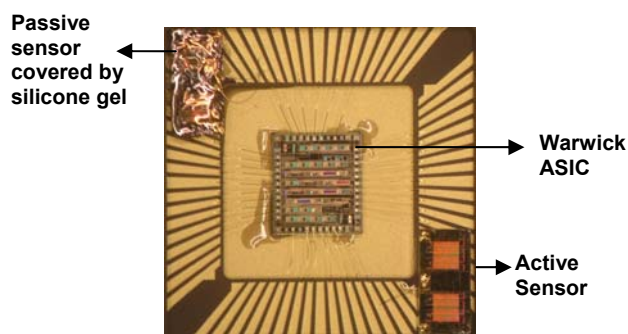
Figure 2. Photograph of the ASIC with the active and passive chemoresistors bonded to it.
