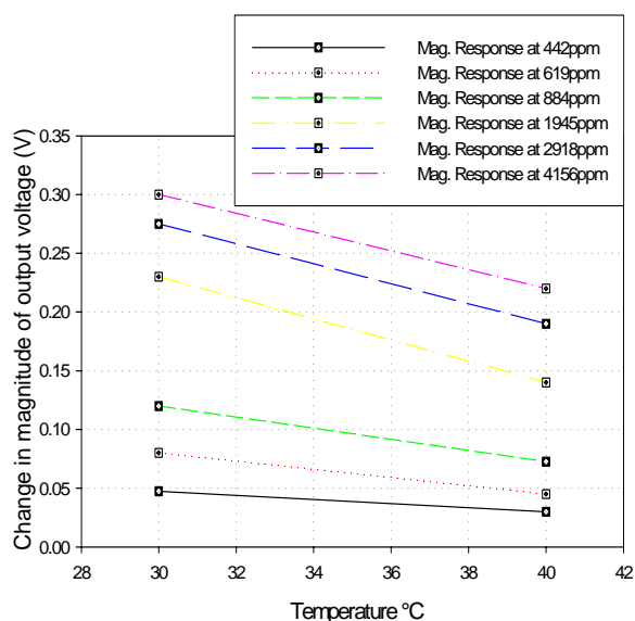
Figure 4. Effect of temperature upon AuNT response of sensor system at six different concentrations of toluene vapour in air at an absolute humidity of 3000 ppm.
