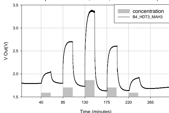
Figure 5. Typical response to toluene vapour at 30°C with 0% rh in duo-type configuration.
