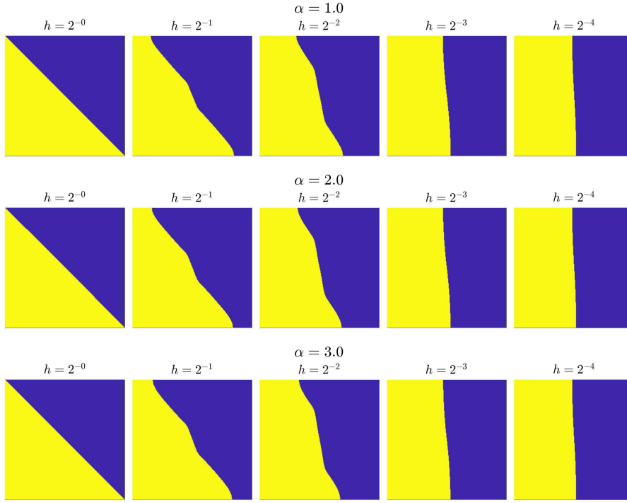
FIG. 4. The sign of minimizers from Figure 3, showing the resulting classification.
