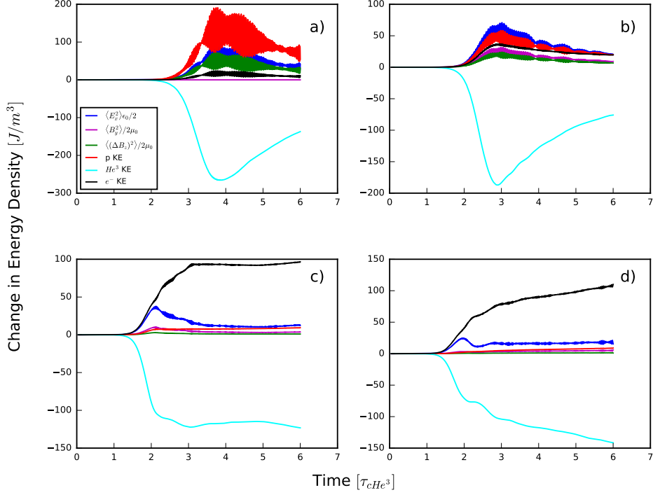
Figure 5.7: Time evolution of the change in energy density of particles and electric and magnetic fields as a function of time for four PIC simulations of the MCI with JET like plasma parameters. Panels a), b), c) and d) correspond to simulations with wave propagation angles equal to 90^\circ , 92^\circ , 94^\circ and 96^\circ respectively. In each panel the parallel component of the ring beam velocity v_{\parallel 0} is set to 0 and time is normalised to the ^3\text{He} gyro-period.
