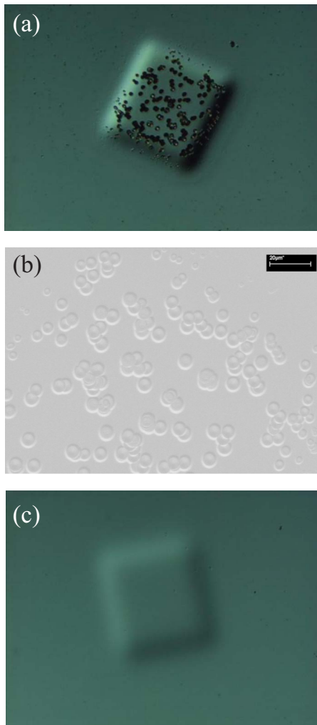
FIG. 5. (Color online) (a) Optical image of the LEPECVD germanium layer showing the large scale topography produced inside the crater by the 750 eV primary beam. (b) 10 keV SEM image of the same crater showing the induced topography change to be pits. (c) An optical image of a 250 eV crater in the LEPECVD germanium showing no topography change.
