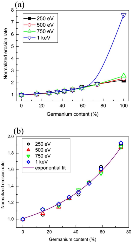
FIG. 6. (Color online) (a) Normalized erosion rates as a function of germanium content for different primary beam energies. (b) Normalized silicon \text{Si}_{1-x}\text{Ge}_x erosion rates and exponential fit as a function of germanium content.
