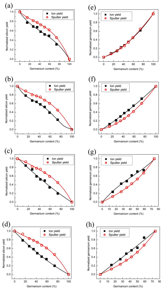
FIG. 8. (Color online) Normalized silicon and germanium ion and sputter yields as a function of germanium content. (a) 250 eV silicon, (b) 500 eV silicon, (c) 750 eV silicon (d) 1 keV silicon, (e) 250 eV germanium, (f) 500 eV germanium, (g) 750 eV germanium, and (h) 1 keV germanium.
