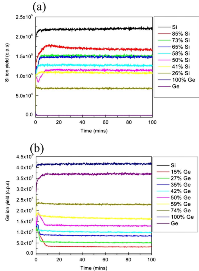
FIG. 2. (Color online) Measured (250 eV) ion yields from the silicon, SiGe, and germanium samples. (a) Silicon ion yields and (b) germanium ion yields.
