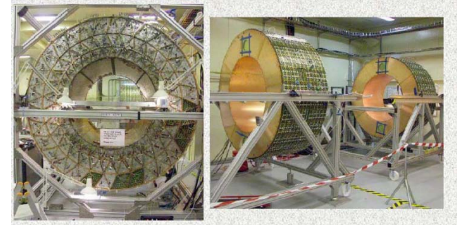
Barrel and endcap TRT
