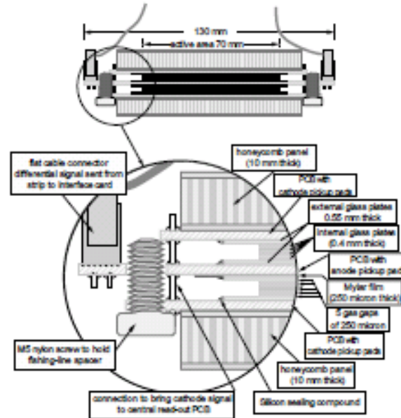
Fig. 1. Cross-section of the MRPC strip for the TOF system of ALICE.
