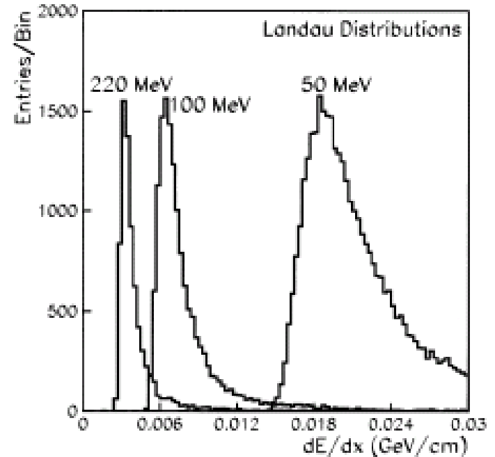
Fig. 1. Landau \langle dE/dx \rangle distributions for pions of momenta 220, 100 and 50 MeV going through 300 \mu m of silicon.
